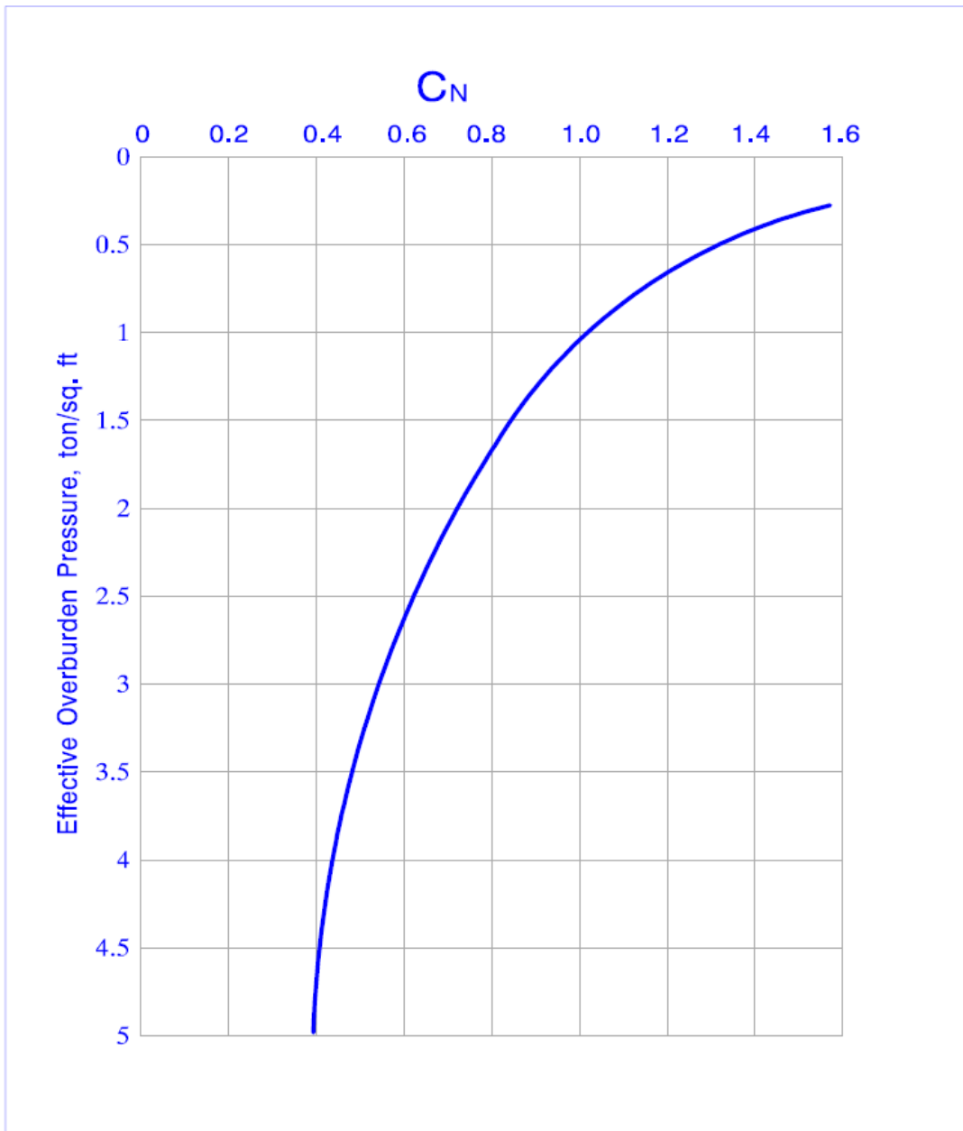
Figure 23 Correlation Between C_N and Effective Overburden Pressure
